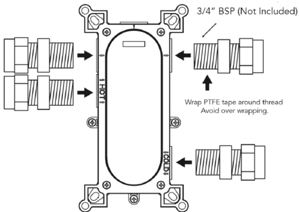
Shower Valve
