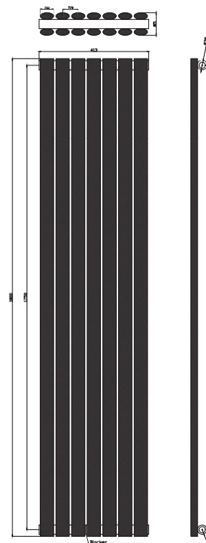
Dimensions (measurements in mm)
