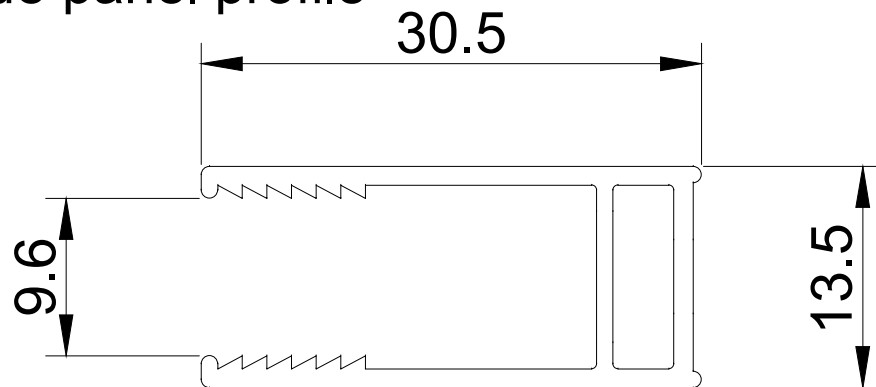
Side panel profile
