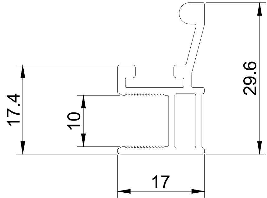
Support arm
