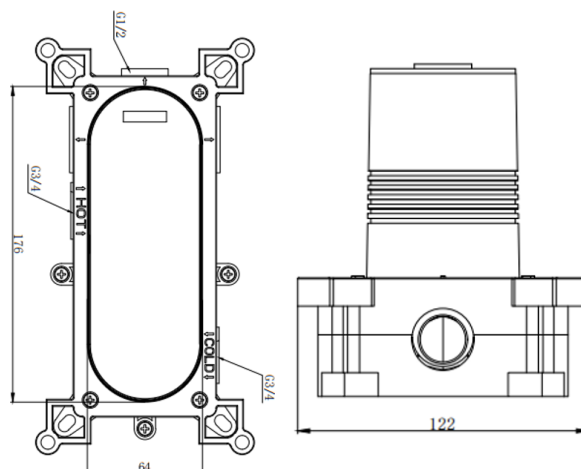
Dimensions (measurements in mm)
