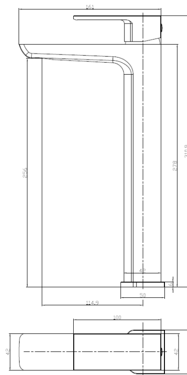
Dimensions (Measurements in mm)
