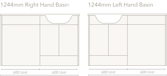
Combined Length of Units 1236mm (inc. end panels)
