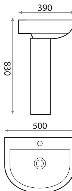
Dimensions (measurements in mm)
